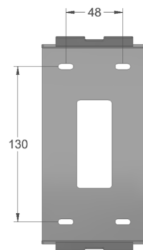
Divar Wall double
